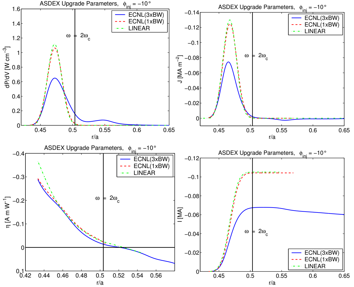
Figure 1: Profiles of the absorbed power density, dP/dV , of the parallel current density, j_{\parallel} , of the current drive efficiency, \eta , and of the total driven current, I , as obtained within linear and nonlinear computations. The indication 3xBW means that the parallel beam width has been increased 3 times.
