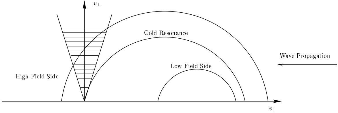
Figure 3: Respective locations of the resonance curves in velocity space for absorption on the low field side, at the cold resonance position and on the high field side. Low and high field side here are defined with respect to the position of the cold resonance surface \omega = 2\omega_c . The cone indicates the region where nonlinear effects of wave-particle interaction are important. Note that in the present case the wave beam is launched from the low field side.
