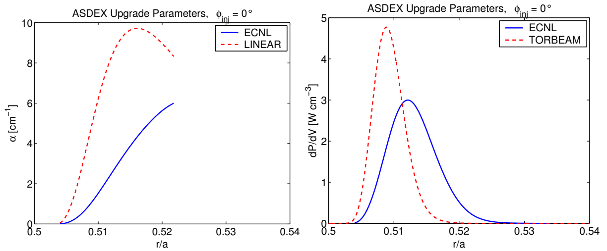
Figure 2: Profiles of the absorption coefficient, \alpha , and of the absorbed power density, dP/dV , as obtained within linear and nonlinear computations for the case of perpendicular launch.
