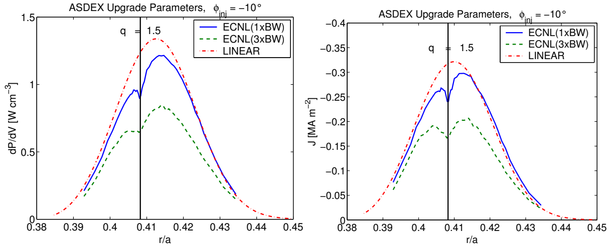
Figure 4: Profiles of the absorbed power density, dP/dV and of the parallel current density, j_{||} as obtained within linear and nonlinear computations for a deposition around the rational surface q = 3/2 . The indication 3xBW means that the parallel beam width has been increased 3 times.
